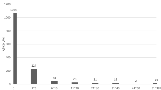
Figure 7: Distribution of Apps in F-Droid by incompatible API usage counts
